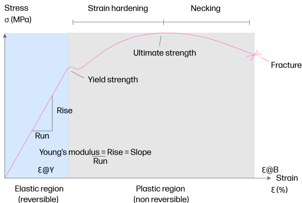
Figure 2. A typical stress-strain curve for a ductile material
