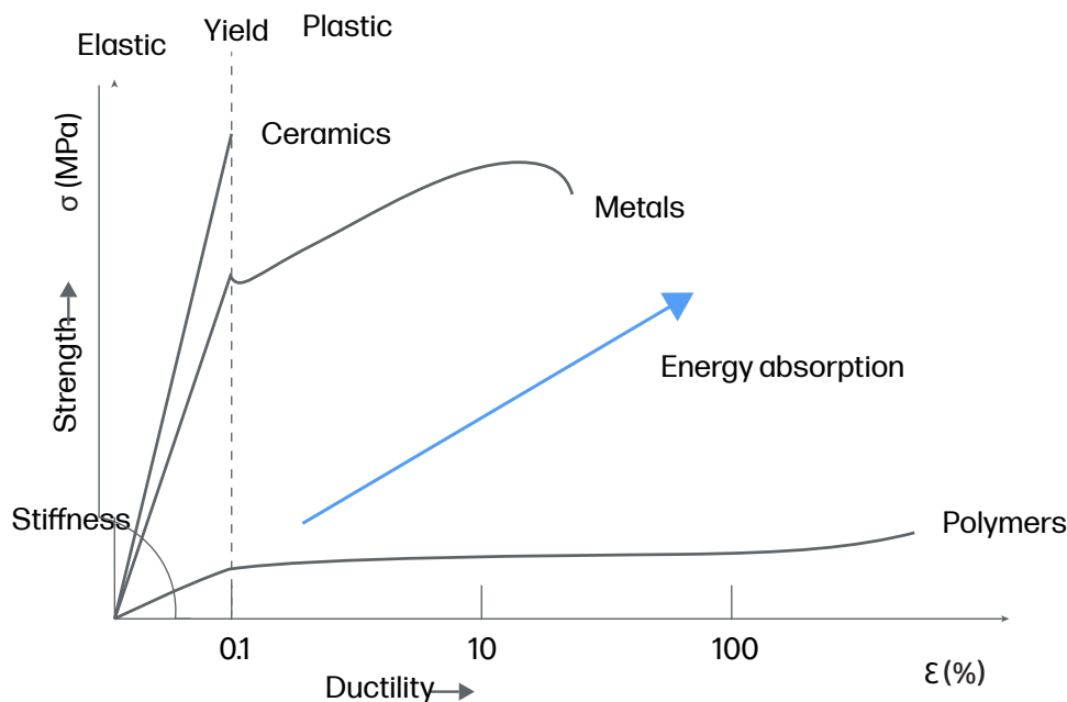
Figure 3. Comparison of polymer, metal, and ceramic materials
